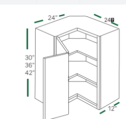
PIE CUT CORNER WPC2430 WPC2436 WPC2442
