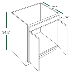
VANITY SINK BASE
