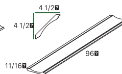
MOLDING CM7
