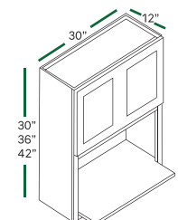
WALL MICROWAVE WM3030 WM3036 WM3042
