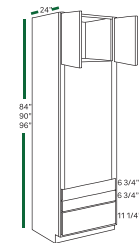
OVEN CABINET OC3384 OC3390 OC3396
