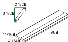
MOLDING CM6
