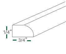
SIMPLE SCRIBE SM8-S
