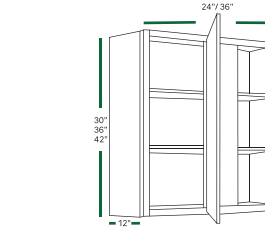
BLIND CORNER WBC2430 WBC2436 WBC2442 WBC3630 WBC3636 WBC3642
