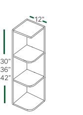
OPEN END OE1230 OE1236 OE1242
